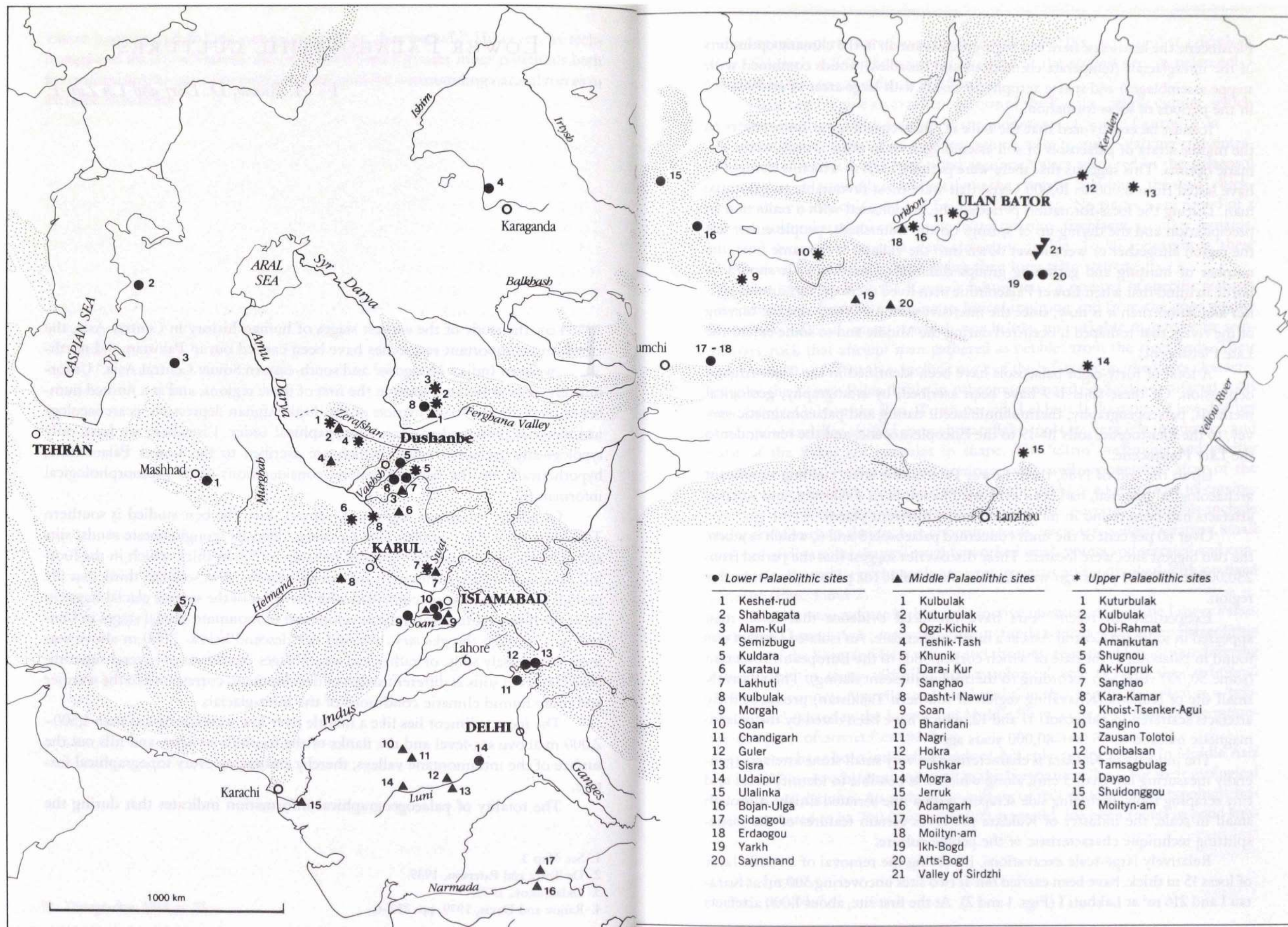
MAP 3. Palaeolithic sites of Central Asia.
