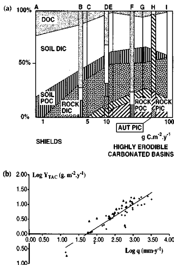
Figure 15.24 Exportation of total carbon by rivers. (a) Decomposition of carbon species exportation in a gradient of total carbon (TC) exportation \text{g C m}^{-2} \text{ y}^{-1} . A = Gambia, B = Zaire, C = Mississippi, D = Solimoes, E = Chiang Jiang, F = Negro, G = Brahmaputra, H = Huang He, I = Dranse. (Data from Meybeck, M. 1993a. C, N, P, and S in rivers: From sources to global inputs, in R. Wollast, F. T. Mackenzie, and L. Chou, eds., Interaction of C, N, P and S Biogeochemical Cycles and Global Change . Springer-Verlag, pp. 163–193.) (b) Yield of riverine total atmospheric carbon ( \text{g C m}^{-2} \text{ y}^{-1} ) vs. runoff ( \text{mm y}^{-1} ) for major rivers. (Data from Meybeck and Ragu 1996, triangles: highly carbonated basins, log-log scale.)
