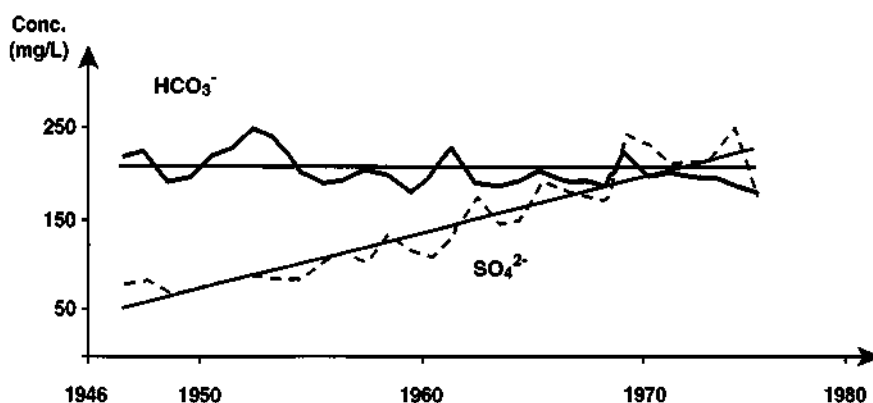
Figure 15.15 Bicarbonate and sulfate trends in the Kura (Caucasus, 188,000 km 2 ). (From Nikanorov and Tsirkunov, 1984.)
