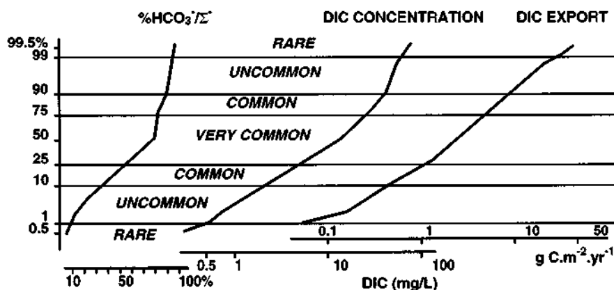
Figure 15.22 Global distribution of DIC concentrations, ionic ratios ( \text{HCO}_3^-/\text{total anions} ), and DIC yields in medium-size pristine basins (vertical scales: probability scale). (From Meybeck, M. 2003b. Global occurrence of major elements in rivers, in K. K. Turekian and H. D. Holland, eds., Treatise of Geochemistry , vol. 5. J. I. Drever, Elsevier, pp. 207–224. With permission.)
