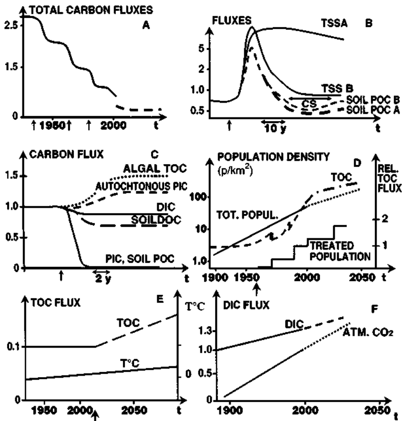
Figure 15.28 Working hypotheses for the contrasted future of carbon fluxes at the Anthropocene. (All fluxes are normalized to pristine average conditions.) (a) Stepwise reduction of fluxes in neorheic rivers with water consumption periods. (b) Stepwise evolution of TSS and soil POC, without proper soil conservation practices (1) and with soil recovery (2); (CS = soil organic carbon sequestration). (c) Contrasted trends after damming (settling vs. autochthonous carbon production). (d) Nonlinear response of river TOC flux downstream of fast-growing megacity with marked time-lag between population growth and urban sewage collection. (e) Threshold TOC increase due to permafrost melt in arctic basins. (f) Gradual DIC increase in forested area due to \text{CO}_2 elevation. (Arrows indicate start of pressure.)
