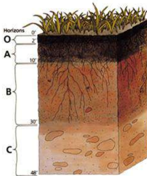
Figure 12.67 Soil Horizons. The R Horizon Would be Below the C Horizon. Image by USDA is in the public domain.
