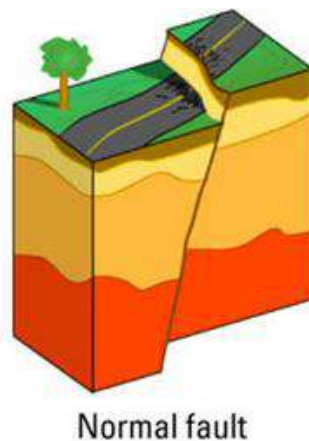
Figure 14.77 Normal Fault Model. Image is in the public domain.
