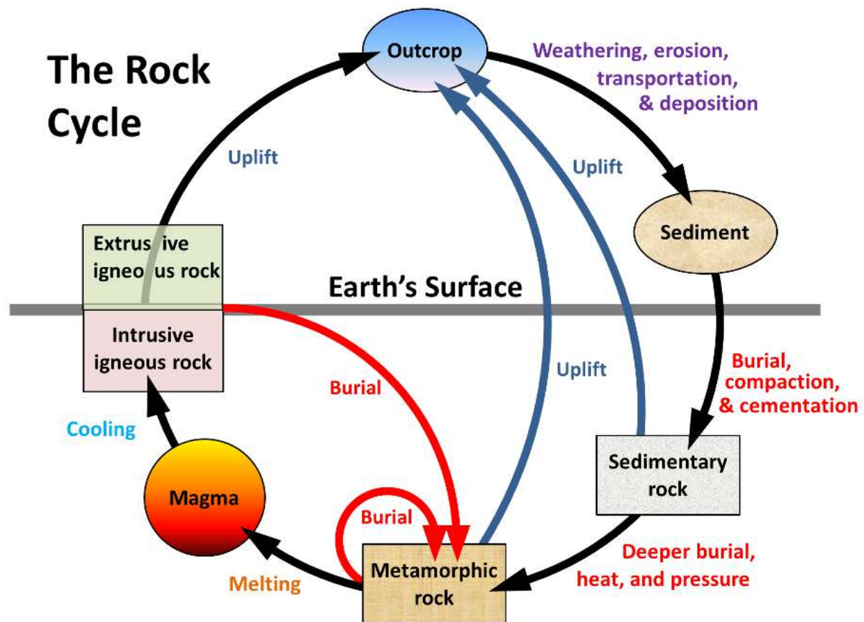
Figure 9.49 The Rock Cycle. Image is used under a Creative Commons Attribution 4.0 International License .
