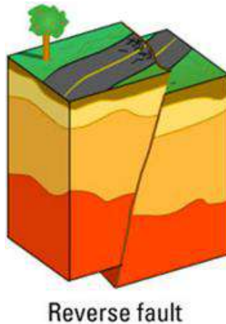
Figure 14.76 Reverse Fault Model. Image is in the public domain.
