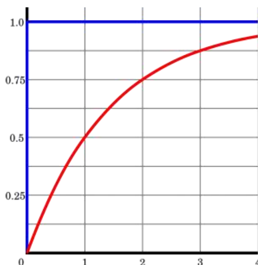
Figure 3.10 Graph of the Number of Half-Lives Image is used under a CC-BY 4.0 license
