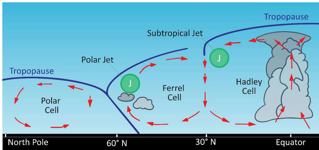
Figure 6.11 The Three Cell Model of Atmospheric Circulation. Image by Anthony Flores is used under a CC-BY-4.0 license.
