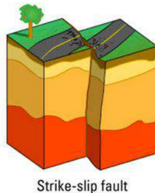
Figure 14.75 Strike-Slip Mode. Image is in the public domain.
