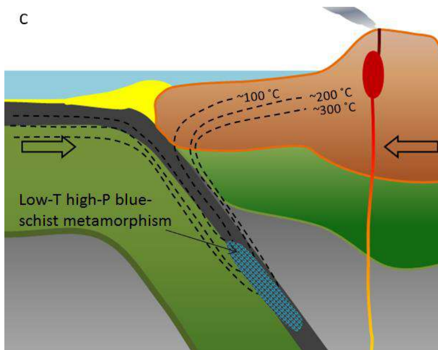
Figure 59 Regional Metamorphism of Oceanic Crust at a Subduction Zone. Image by Steven Earl is used under a Creative Commons Attribution 4.0 International License .
