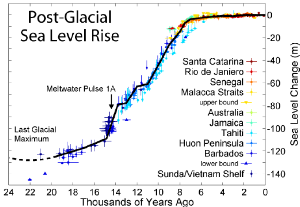
Figure 16.98 Eustatic Sea-Level Curve for the Past 24 ka. Sea-Level rise is Global due to Melting Glaciers. Graph from Wikimedia Foundation Inc., CC BY-SA 3.0 .
