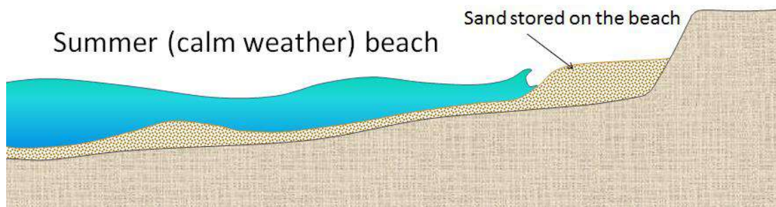
Figure 16.95 The Differences Between Summer & Winter on Beaches in Areas Where the Winter Conditions are Rougher & Waves Have a Shorter Wavelength but Higher Energy. In winter, Sand from the Beach is Stored Offshore in Sand Bars. Image by Steven Earle, CC BY 4.0 .
