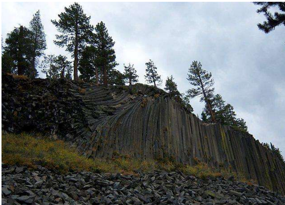
Figure 15.5 Columnar Basalt at The Devils Postpile Near Mammoth, California. Image by Jeremy Patrich is used under a CC-BY 4.0 license.
