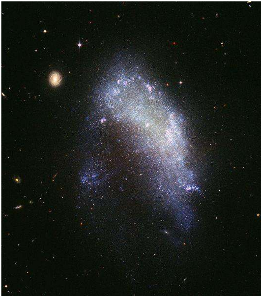
Figure 2.15 An Irregularly Shaped Galaxy. Image by NASA is in the public domain.
