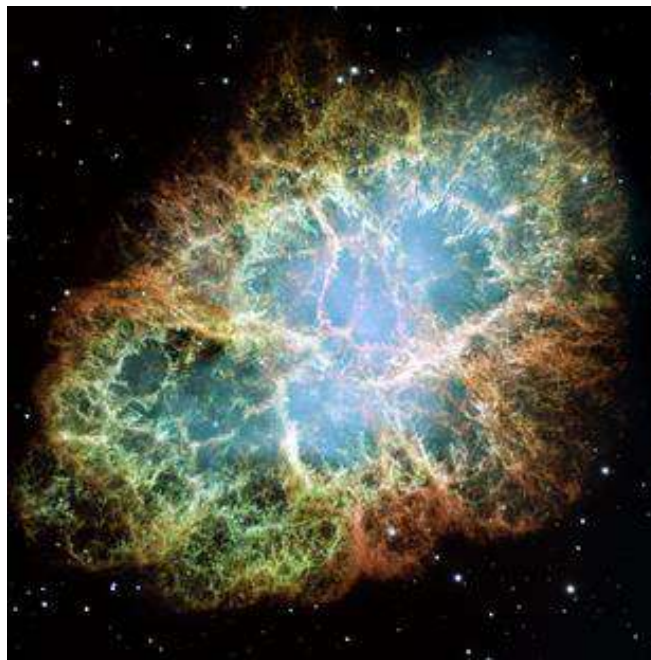
Figure 2.21 Image of the Crab Nebula. Image by NASA is in the public domain.
