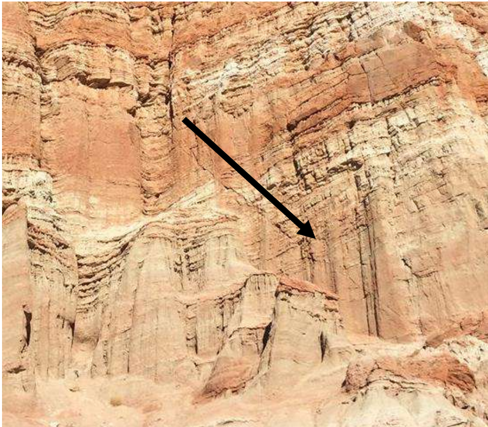
Figure 14.74 The Offset-- or Faulting in Red Rock State Park, in Cantil California. Image by Jeremy Patrich is used under a CC-BY 4.0 license.
