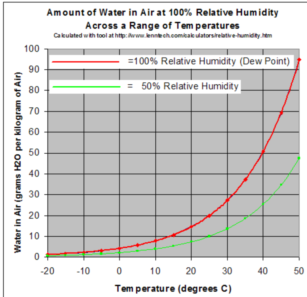
Figure 7.34 Diagram Explaining the Calculation of Relative Humidity.
