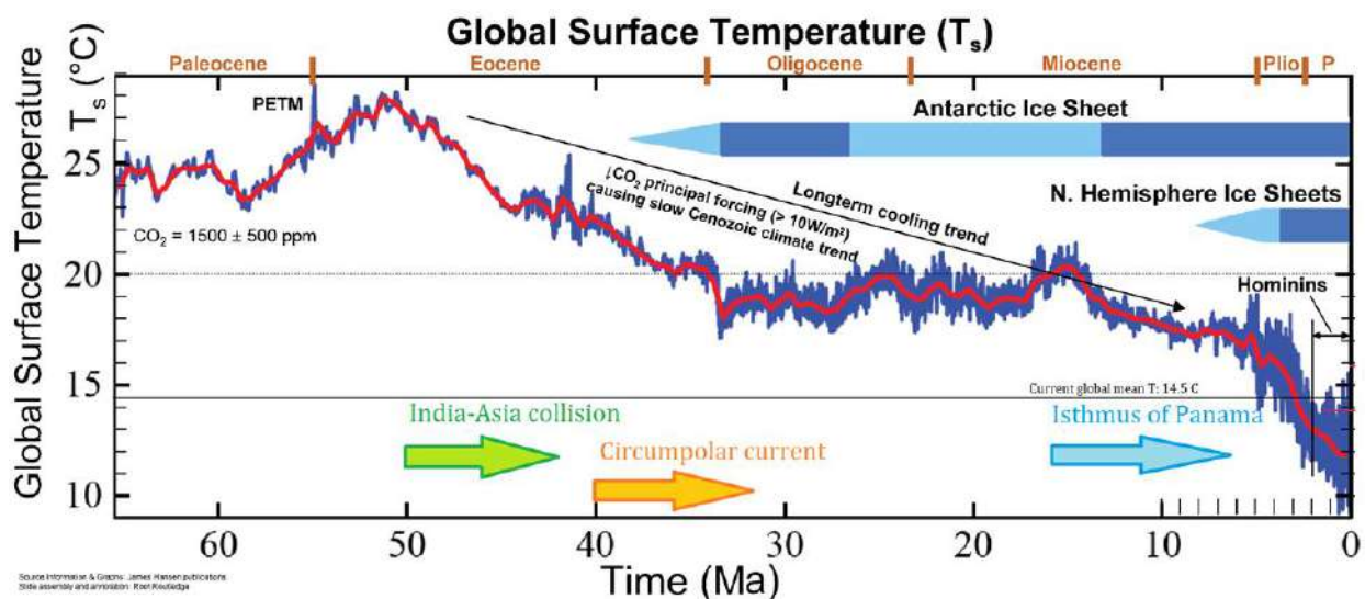
Figure 19.132 The Global Temperature Trend over the Past 65 Ma, the Cenozoic. Image by Steven Earle, CC BY 4.0 .
