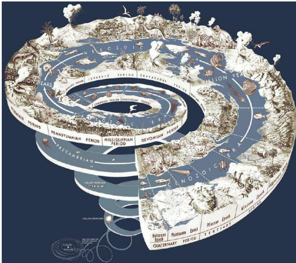
Figure 3.7 Geological Time Spiral. Image is in the public domain.
