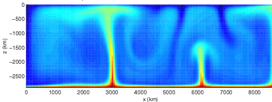
Figure 13.5 This is a Snapshot of One Time-Step in a Model of Mantle Convection. Image is used under a Attribution-Share Alike 3.0 Unported license.
