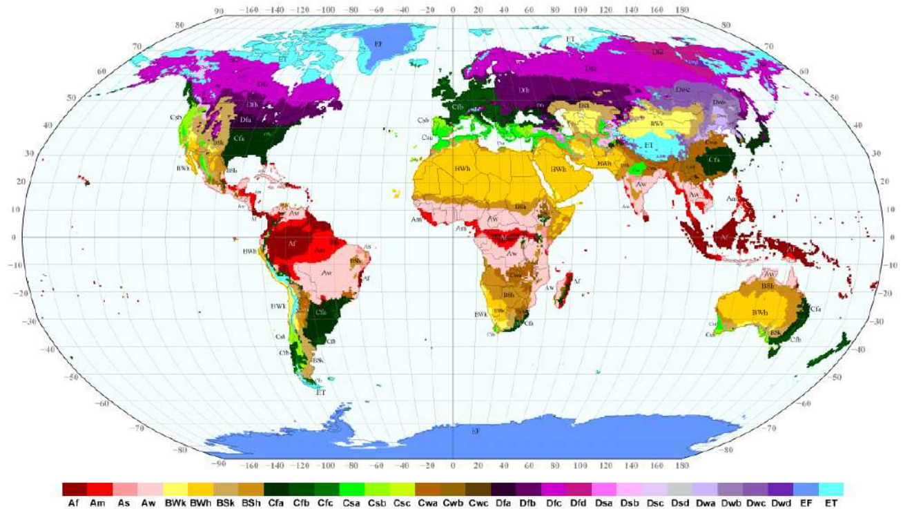
Figure 7.10 Köppen-Geiger Climate Subdivisions. Image is in the public domain.
