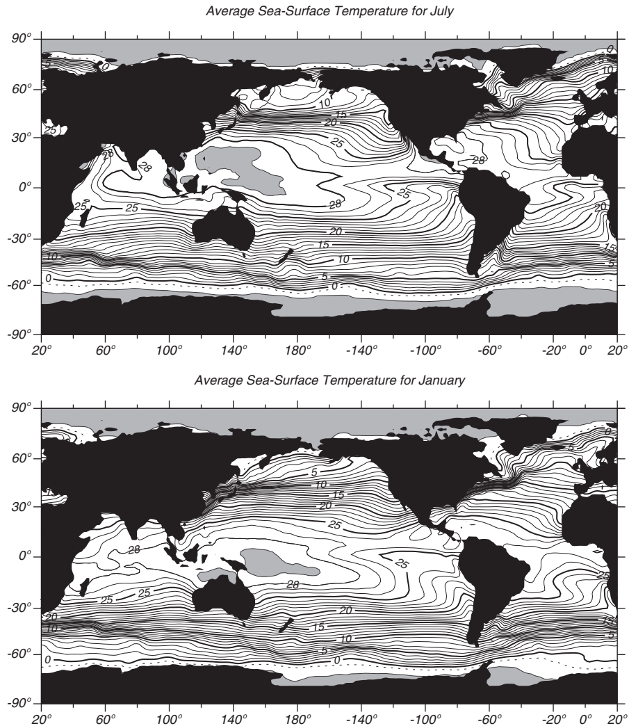
Figure 6.2 Mean sea-surface temperature calculated from the optimal interpolation technique (Reynolds and Smith, 1995) using ship reports and AVHRR measurements of temperature. Contour interval is 1°C with heavy contours every 5°C. Shaded areas exceed 29°C.
