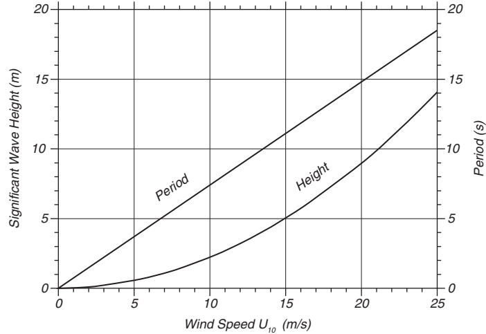
Figure 16.8 Significant wave height and period at the peak of the spectrum of a fully developed sea calculated from the Pierson-Moskowitz spectrum using (16.35 and 16.32).
