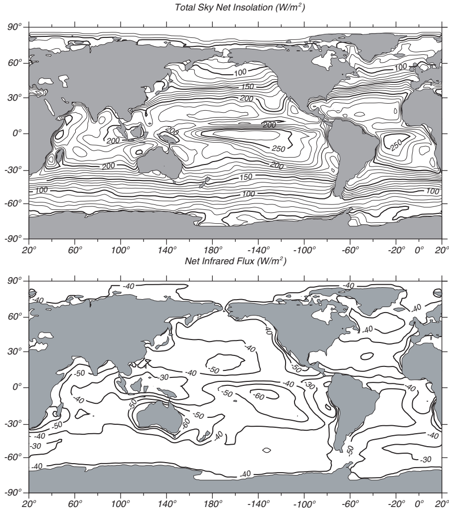
Figure 5.8 Annual-mean insolation Q_{SW} ( top ) and infrared radiation Q_{LW} ( bottom ) through the sea surface during 1989 calculated by the Satellite Data Analysis Center at the NASA Langley Research Center (Darnell et al., 1992) using data from the International Satellite Cloud Climatology Project. Units are \text{W/m}^2 , contour interval is 10 \text{ W/m}^2 .
