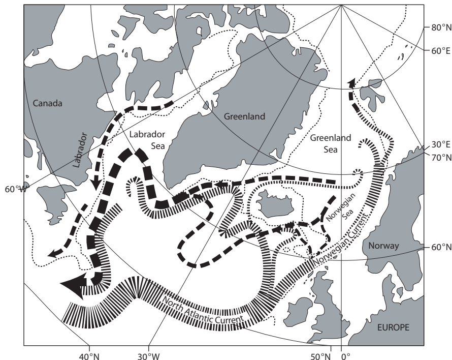
Figure 13.1 The surface (narrow dashes) and deep (wide dashes) currents in the north Atlantic. The North Atlantic Current brings warm water northward where it cools. Some sinks and returns southward as a cold, deep, western-boundary current. Some returns southward at the surface. From Woods Hole Oceanographic Institution.
