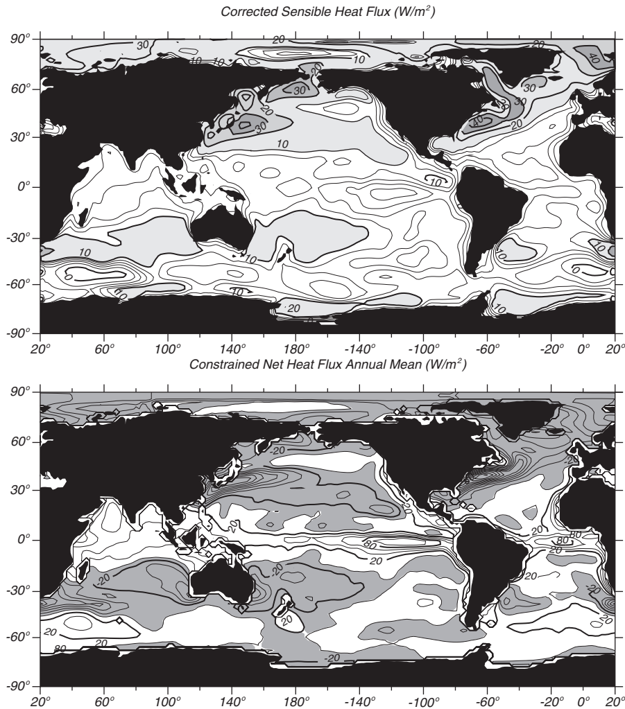
Figure 5.10 Annual-mean upward sensible heat flux Q_S ( top ) and constrained, net, downward heat flux ( bottom ) through the sea surface in \text{W/m}^2 calculated by DaSilva, Young, and Levitus (1995) using the ICOADS data set from 1945 to 1989. Contour interval is 2 \text{ W/m}^2 (top) and 20 \text{ W/m}^2 (bottom).
