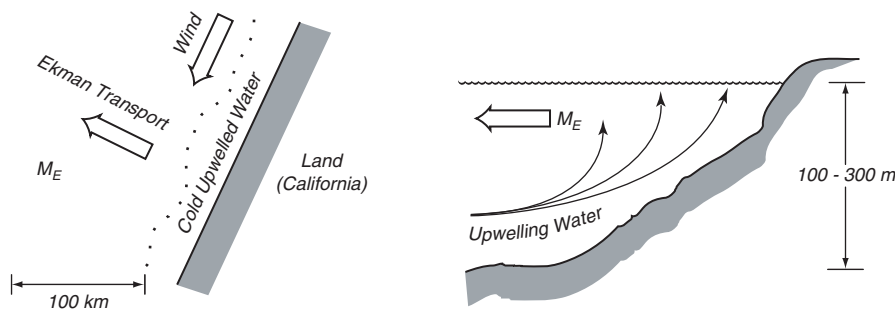
Figure 9.8 Sketch of Ekman transport along a coast leading to upwelling of cold water along the coast. Left: Plan view. North winds along a west coast in the northern hemisphere cause Ekman transports away from the shore. Right: Cross section. The water transported offshore must be replaced by water upwelling from below the mixed layer.
