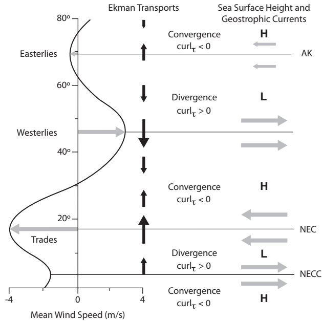
Figure 12.8 An example of how winds produce geostrophic currents running upwind. Ekman transports due to winds in the north Pacific ( Left ) lead to Ekman pumping ( Center ), which sets up north-south pressure gradients in the upper ocean. The pressure gradients are balanced by the Coriolis force due to east-west geostrophic currents ( Right ). Horizontal lines indicate regions where the curl of the zonal wind stress changes sign. AK : Alaskan Current, NEC : North Equatorial Current, NECC : North Equatorial Counter Current.
