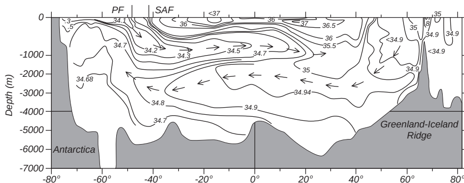
Figure 13.10 Contour plot of salinity as a function of depth in the western basins of the Atlantic from the Arctic Ocean to Antarctica. The plot clearly shows extensive cores, one at depths near 1000 m extending from 50°S to 20°N, the other at is at depths near 2000 m extending from 20°N to 50°S. The upper is the Antarctic Intermediate Water, the lower is the North Atlantic Deep Water. The arrows mark the assumed direction of the flow in the cores. The Antarctic Bottom Water fills the deepest levels from 50°S to 30°N. PF is the polar front, SAF is the subantarctic front. See also figures 10.15 and 6.10. After Lynn and Reid (1968).
