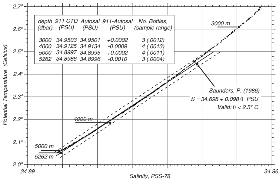
Figure 6.15. Results from a test of the Sea-Bird Electronics 911 Plus CTD in the North Atlantic Deep Water in 1992. Data were collected at 43.17^\circ \text{ N} and 14.08^\circ \text{ W} from the R/V Poseidon. From Sea-Bird Electronics (1992).
