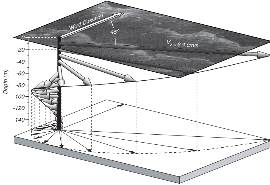
Figure 9.3. Ekman current generated by a 10 m/s wind at 35^\circ N.
