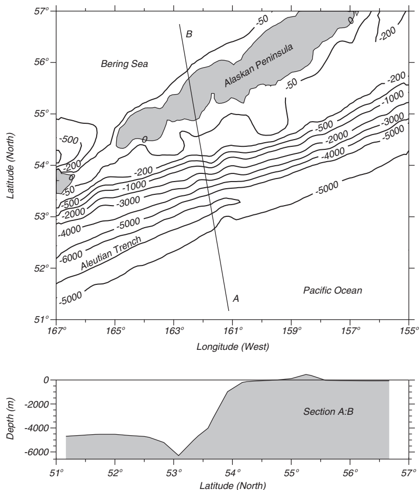
Figure 3.9 An example of a trench, the Aleutian Trench; an island arc, the Alaskan Peninsula; and a continental shelf, the Bering Sea. The island arc is composed of volcanoes produced when oceanic crust carried deep into a trench melts and rises to the surface. Top: Map of the Aleutian region of the North Pacific. Bottom: Cross-section through the region.
