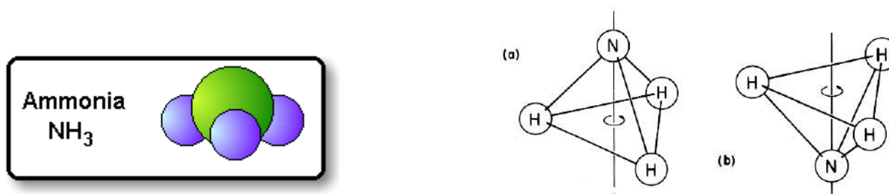
Fig 12: The Ammonia molecule. LEFT: basic structure, with a Nitrogen atom above a triangle of Hydrogen atoms. RIGHT: The N atom can also lie below the \text{H}_3 triangle, and tunnels between the 2 configurations (a) and (b).
