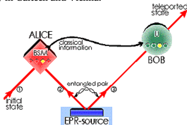
Fig 31: The basic design for quantum teleportation, in which Alice at A teleports to Bob at B a quantum state (the initial state shown) by entangling it with an ‘entangled pair state’ which is shared by Alice and Bob (see text).
