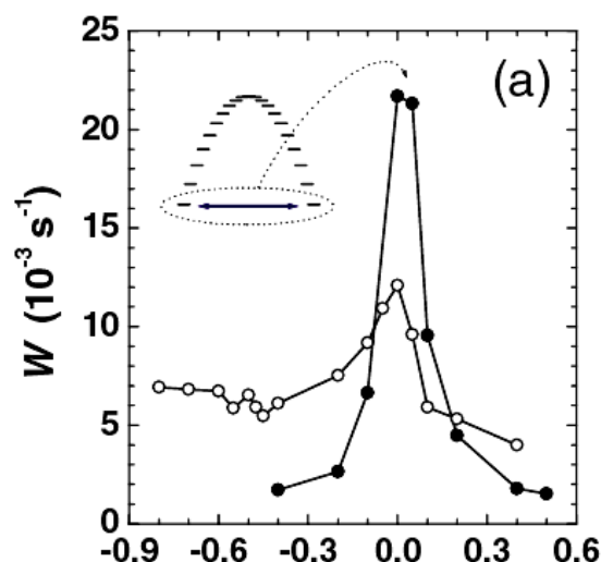
Fig 30: The effects of decoherence. LEFT: A superconducting SQUID scans through different tunneling splittings, & ‘resonates’ with different environmental 2-state systems- disrupting its behaviour (Martinis et al, Santa Barbara). RIGHT: The nuclear spin environment entangles with a magnetic molecular spin, & its relaxation rate W is radically increased (Morello et al, Leiden)
