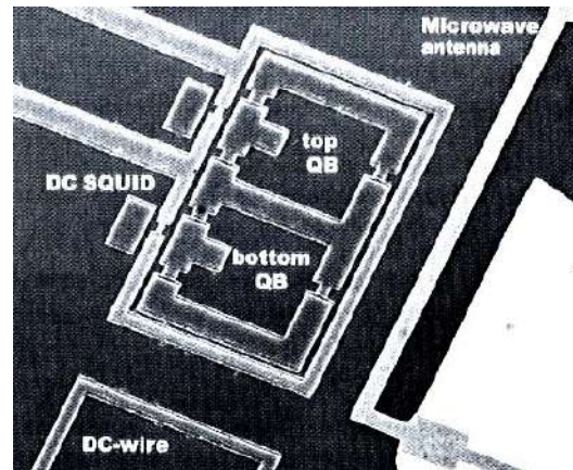
Fig. 25: Operating designs for entangled pair of superconducting qubits. LEFT: pair of Cooper pair boxes (Nakamura, Tokyo, 2003); note scale at bottom. RIGHT: Pair of SQUIDs (Delft, 2002)
