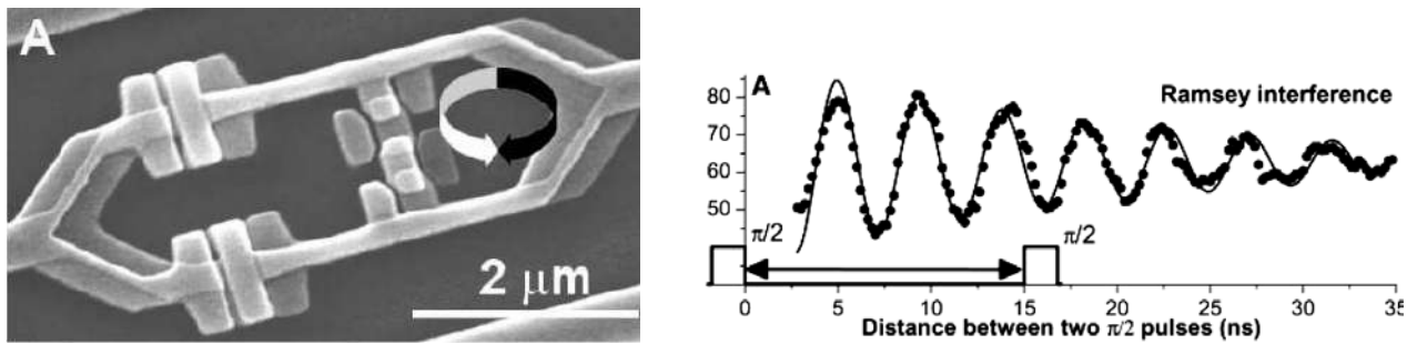
Fig. 24: A superconducting ‘qubit’ (Delft lab). LEFT: the qubit- the 2 states have currents circulating in opposite directions. RIGHT: interference between current states at different times, as the system oscillates from one current state to another.
