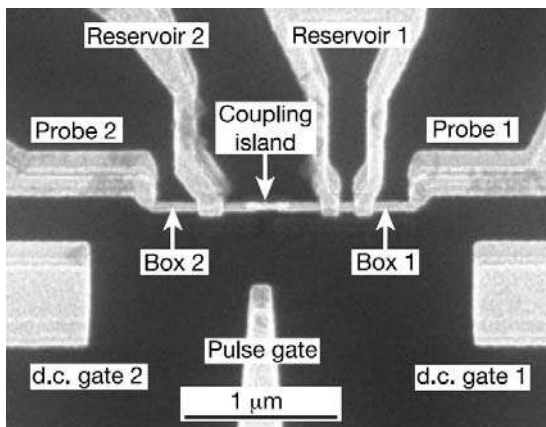
Fig. 25: Operating designs for entangled pair of superconducting qubits. LEFT: pair of Cooper pair boxes (Nakamura, Tokyo, 2003); note scale at bottom. RIGHT: Pair of SQUIDs (Delft, 2002)
