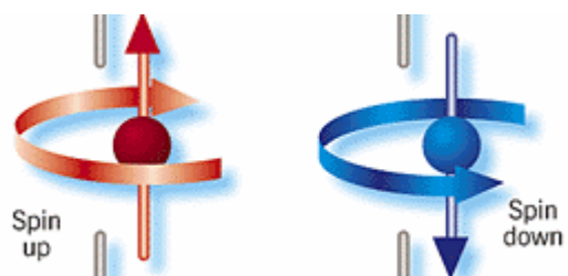
Fig 7: A 2-state spin system- the 2 states behave as though they have circulating currents (in opposite directions), which generate small magnetic fields (which are either up or down)
