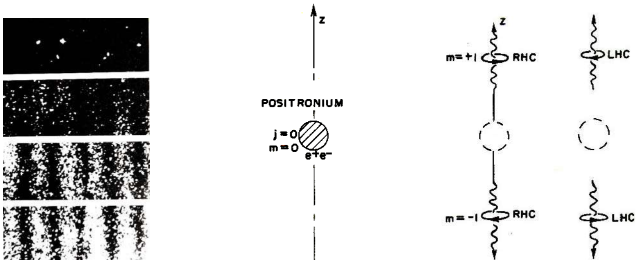
Fig. 9: Quantum properties of light/photons. LEFT: How the 2-slit interference pattern develops in time, as more and more photons arrive. RIGHT: Decay of zero-spin positronium into 2 photons moving in opposite directions. 2 final states are possible- one with helicities m = +1, -1 for photons moving up/down, and the other with the opposite helicities, ie., m = -1, +1 respectively.
