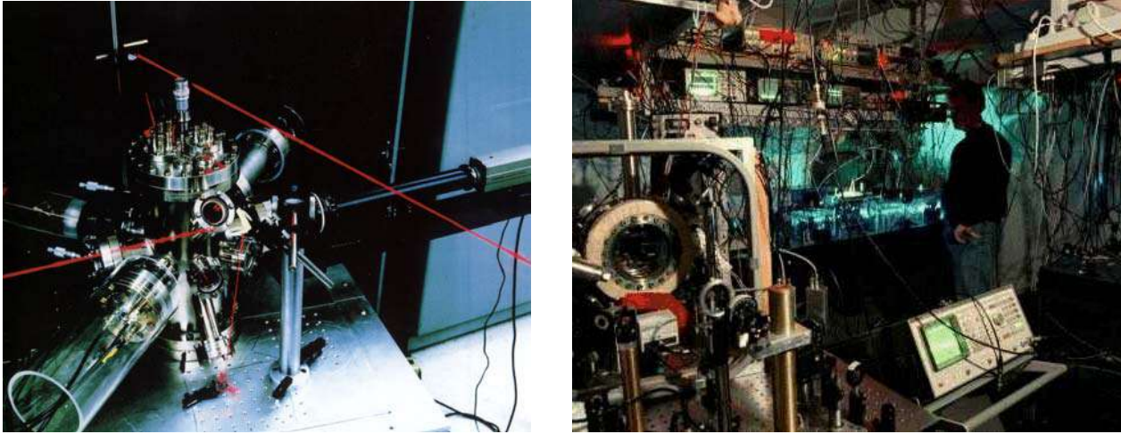
Fig 32: scenes from a quantum optics lab: LEFT: a set-up in which 2 qubits are being remotely entangled by lasers. RIGHT: The lab of E Polzik (Copenhagen).
