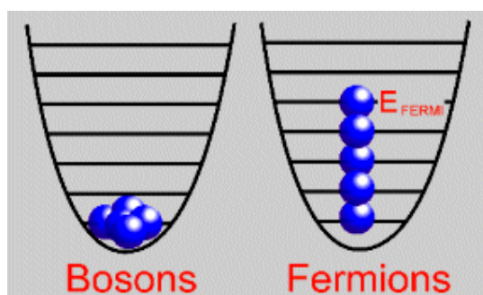
Fig 5: How bosons and fermions will fill up quantum states differently (see text)
