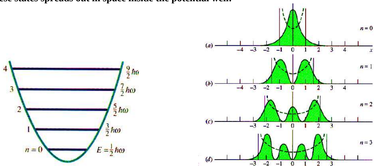
Fig 4: Bound states in a potential well. LEFT: the well, with energy levels shown as horizontal lines. RIGHT: the probability to find the particle at some position relative to the bottom of the well (the lowest energy position), for the lowest ground state ( n=0 ) and the first few excited states.
