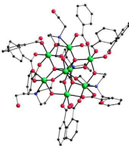
Fig. 26: Qubits from magnetic molecules. LEFT: The 'Fe-8' molecule, widely studied as a possible magnetic qubit (Morello, UBC). RIGHT: A quantum 'spin net' of 'Mn 4 ' molecules- this is a set of
