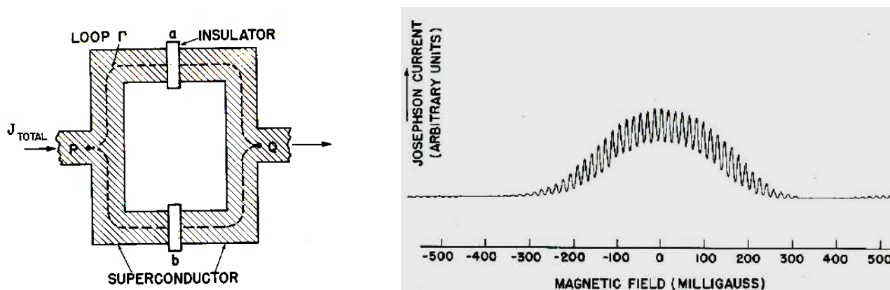
Fig 10: The ‘SQUID’. LEFT: schematic SQUID- electrons come in at left, travel through the 2 arms, via the insulating ‘Josephson junctions’ a and b, and out to the right. RIGHT: The current coming out of the SQUID as a function of the magnetic field through the SQUID.
