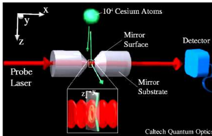
Fig 29: An example of a cavity QED set-up, from Caltech. The atoms fall into the cavity, are held there for some time by focused high-intensity laser light before falling out.
