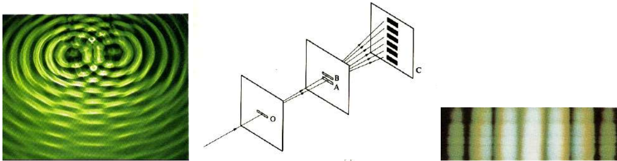
Fig 8: Wave properties of light. LEFT: interference between waves from 2 sources. CENTRE: the 2-slit interference experiment. RIGHT: Experimental 2-slit interference from a green light source.
