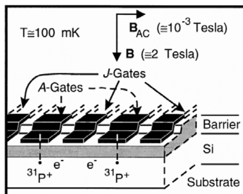
Fig 27: The Sydney/Maryland design for a spin qubit computer (the P ions) in a semiconductor
