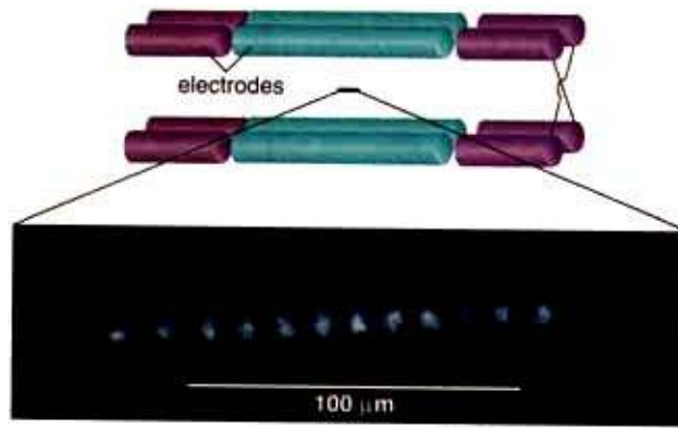
Fig 28: the interior of a linear ion trap: we see 11 ions held in position by the electric fields from the surrounding electrodes (and imaged optically).
