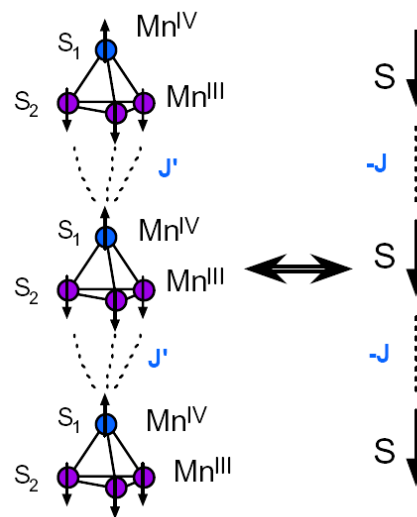
Fig. 26: Qubits from magnetic molecules. LEFT: The 'Fe-8' molecule, widely studied as a possible magnetic qubit (Morello, UBC). RIGHT: A quantum 'spin net' of 'Mn 4 ' molecules- this is a set of
