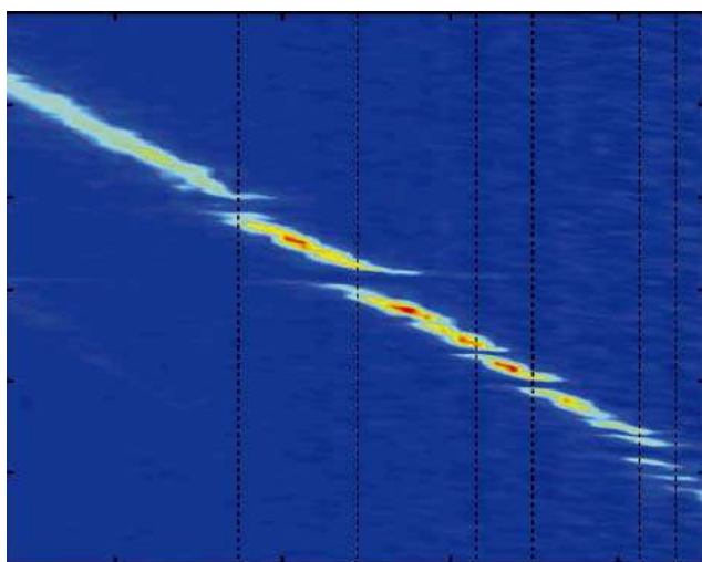
Fig 30: The effects of decoherence. LEFT: A superconducting SQUID scans through different tunneling splittings, & ‘resonates’ with different environmental 2-state systems- disrupting its behaviour (Martinis et al, Santa Barbara). RIGHT: The nuclear spin environment entangles with a magnetic molecular spin, & its relaxation rate W is radically increased (Morello et al, Leiden)
