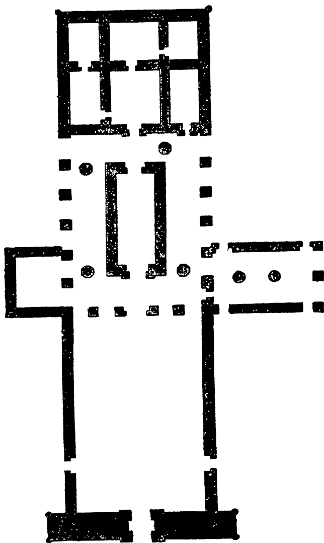
GROUND-PLAN OF TEMPLE AT MEDINET-ABOU.
